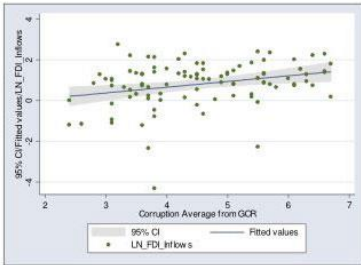
Figure 2: Corruption and FDI Inflows with a fitted regression line
